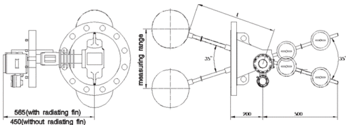
UQD.A-90 UQD.Z-90 Outline sketch and Installation Dimensions of Ordinary Type
